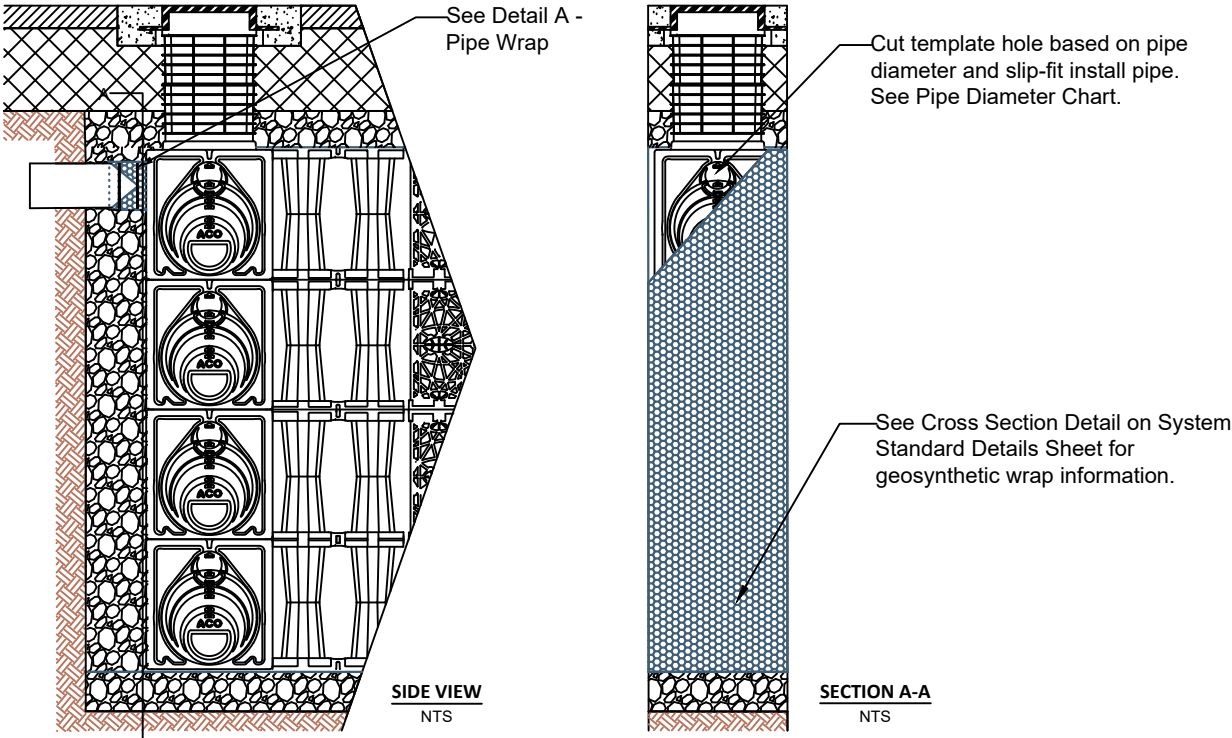
4.0 LAYER 600HD - REMOTE ACCESS UNIT PIPE INSTALLATION
