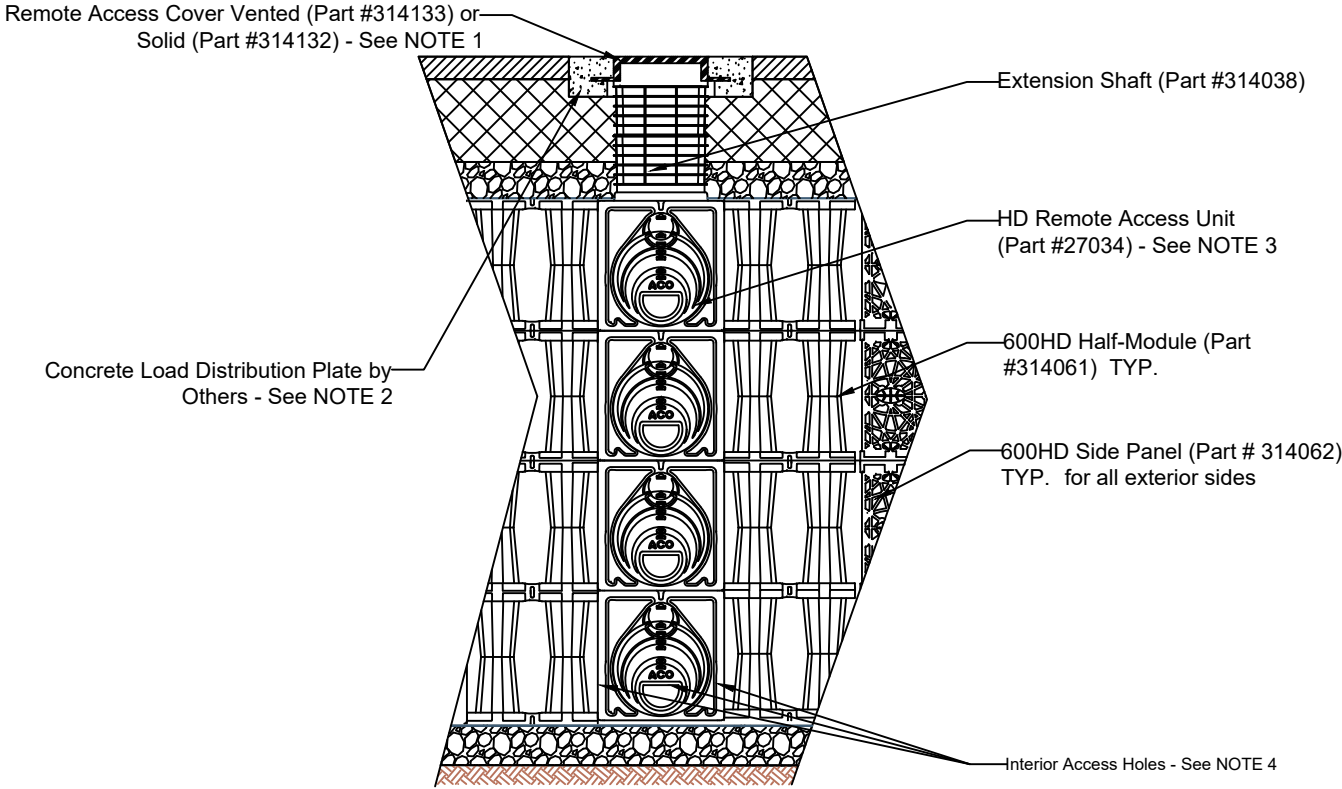
4.0 LAYER 600HD - REMOTE ACCESS UNIT CROSS SECTION
