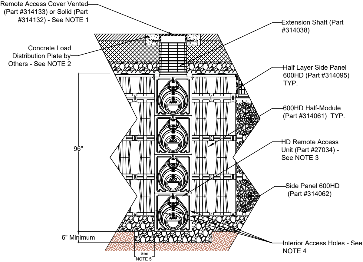
3.5 LAYER 600HD - REMOTE ACCESS UNIT CROSS SECTION NTS
