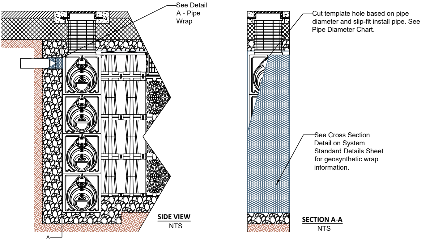
3.5 LAYER 600HD - REMOTE ACCESS UNIT PIPE INSTALLATION NTS
