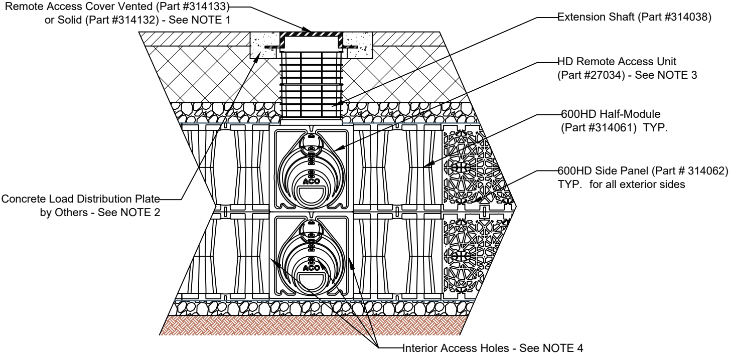
2.0 LAYER 600HD - REMOTE ACCESS CROSS SECTION
