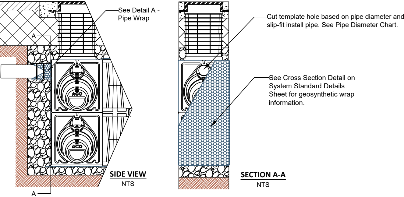
2.0 LAYER 600HD - REMOTE ACCESS UNIT PIPE INSTALLATION
