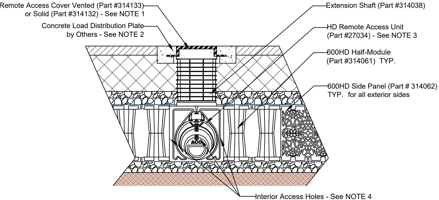
1.0 LAYER 600HD - REMOTE ACCESS UNIT CROSS SECTION
