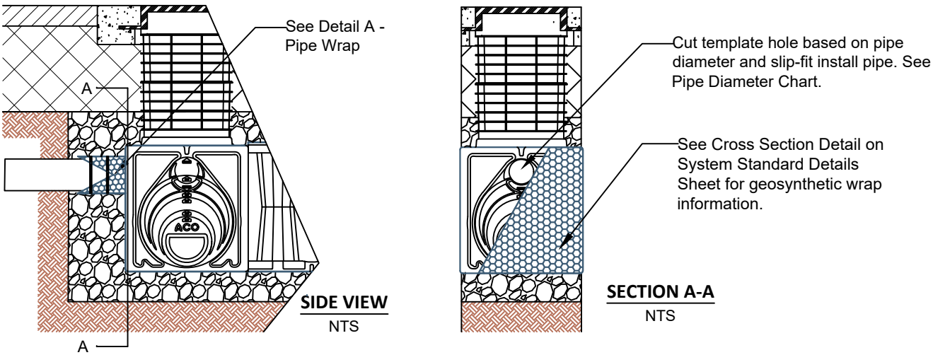
1.0 LAYER 600HD - REMOTE ACCESS UNIT PIPE INSTALLATION
