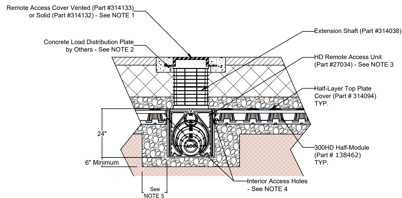
0.5 LAYER 300HD REMOTE ACCESS UNIT CROSS SECTION NTS
