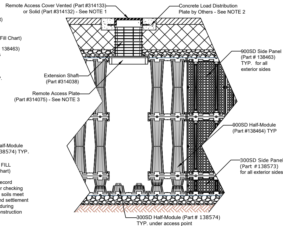
2 LAYER 900SD - 1 LAYER 300SD ACCESS POINT CROSS SECTION
