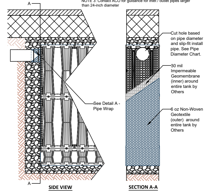
2 LAYER 900SD - 1 LAYER 300SD PIPE INSTALLATION
