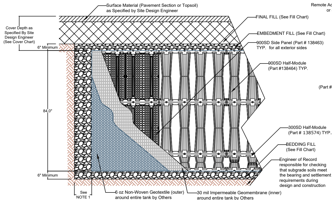
2 LAYER 900SD - 1 LAYER 300SD DETENTION CROSS SECTION
