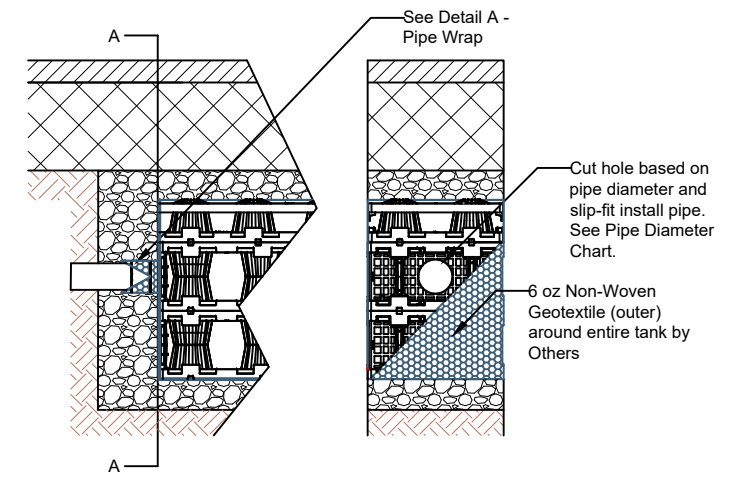
2.5 LAYER 300SD PIPE INSTALLATION NTS
