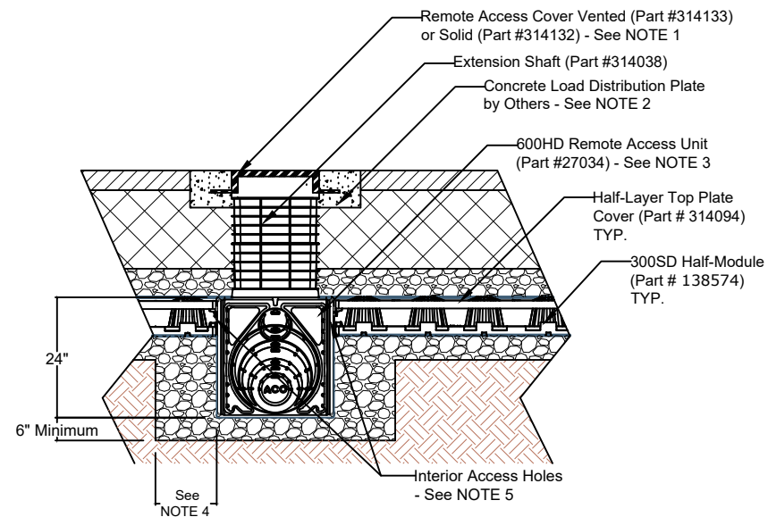
0.5 LAYER 300SD ACCESS UNIT CROSS SECTION
