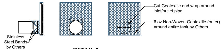
DETAIL A PIPE WRAP
