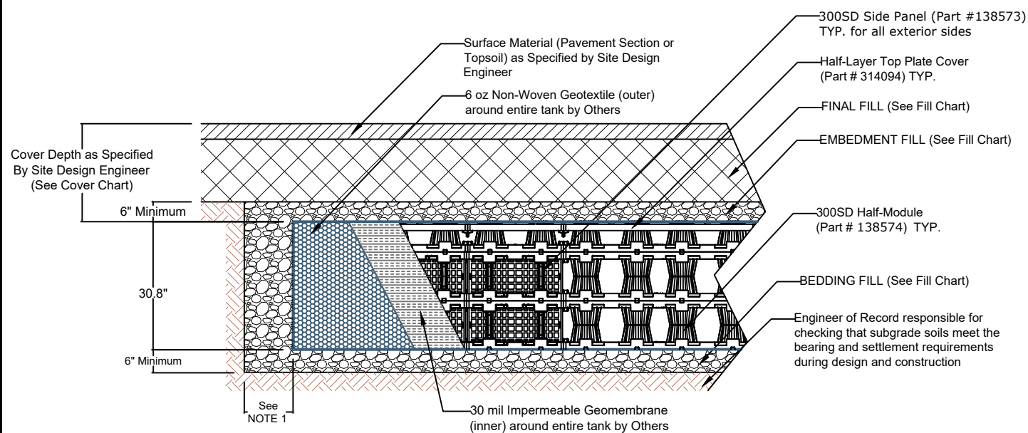
2.5 LAYER 300SD DETENTION CROSS SECTION NTS
