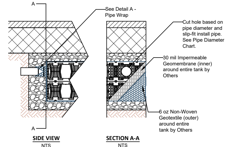
2 LAYER 300SD PIPE INSTALLATION NTS
