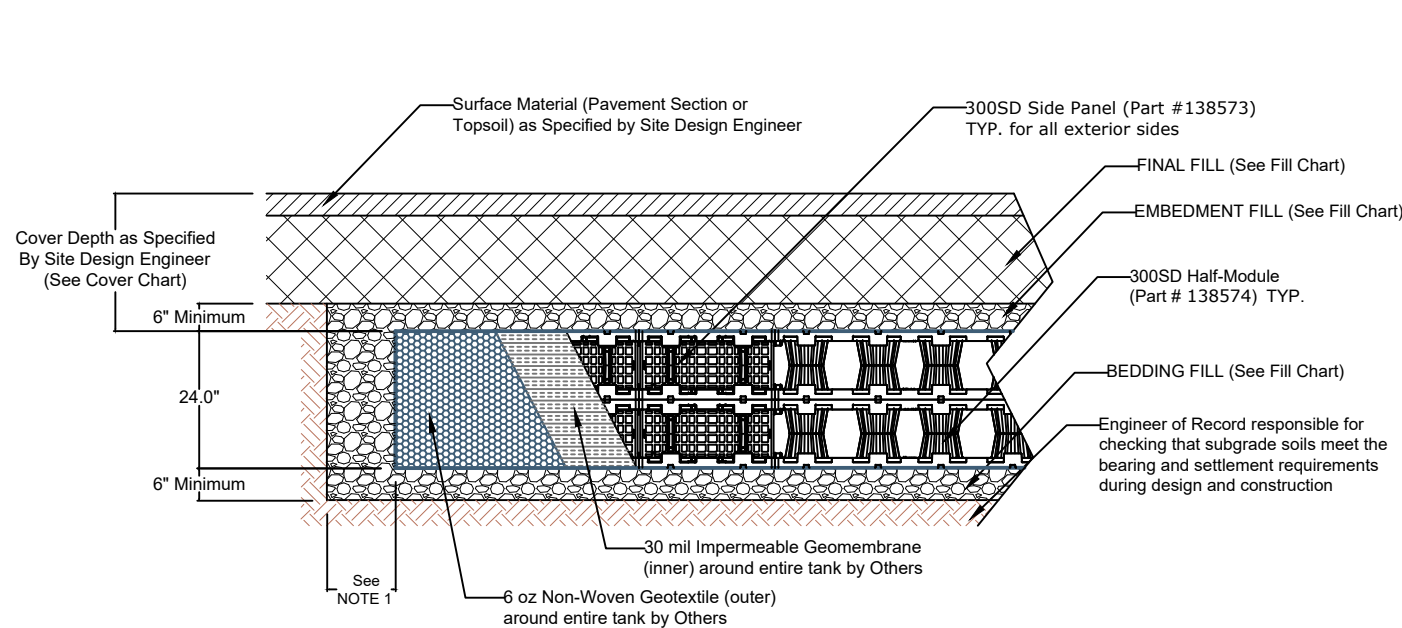
2 LAYER 300SD DETENTION CROSS SECTION NTS
