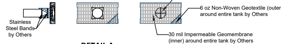
DETAIL A PIPE WRAP NTS
