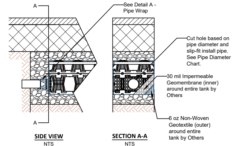
1.5 LAYER 300SD PIPE INSTALLATION NTS
