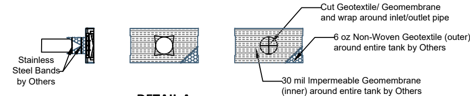
DETAIL A PIPE WRAP NTS
