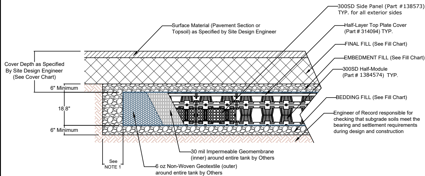
1.5 LAYER 300SD DETENTION CROSS SECTION NTS
