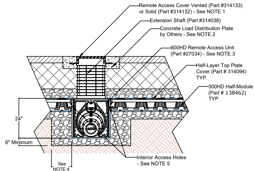
0.5 LAYER 300HD ACCESS UNIT CROSS SECTION NTS
