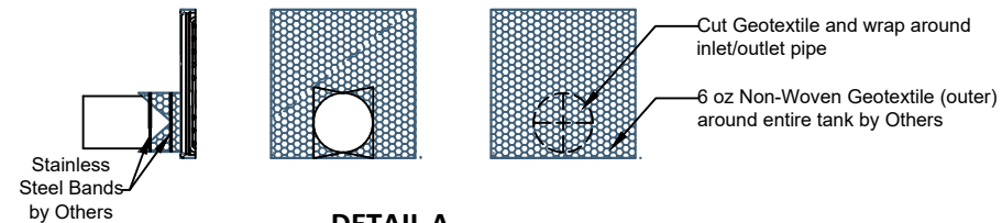
DETAIL A PIPE WRAP NTS
