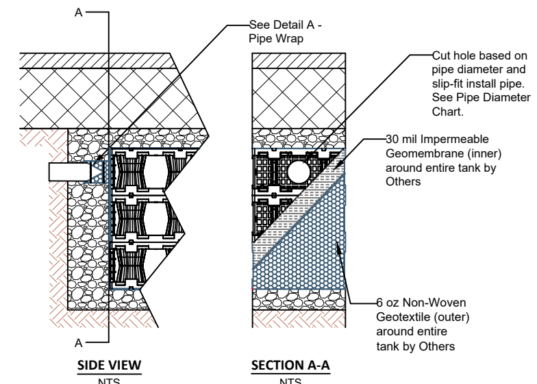
3 LAYER 300HD PIPE INSTALLATION NTS
