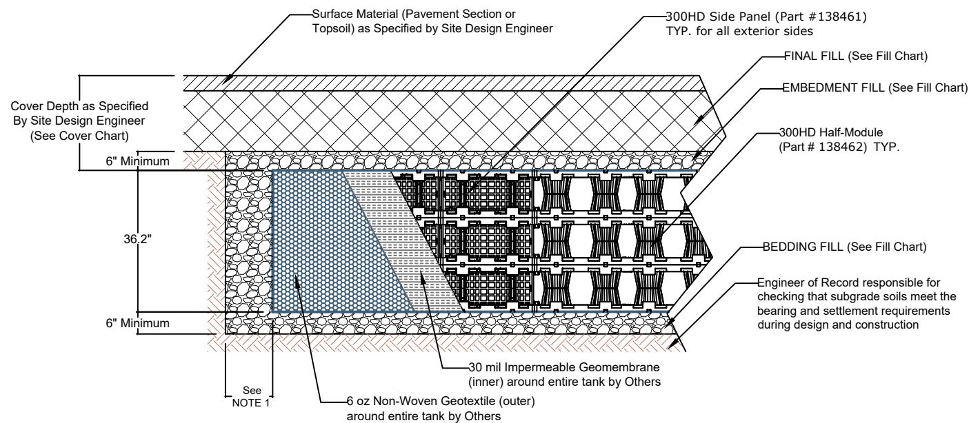
3 LAYER 300HD DETENTION CROSS SECTION NTS
