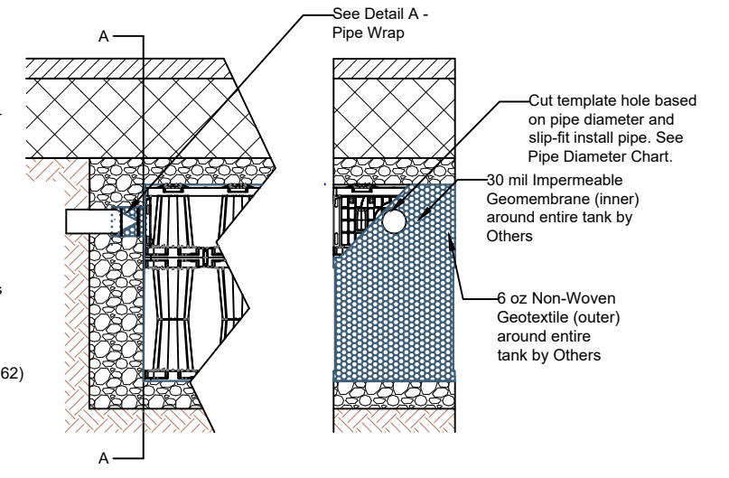
1.5 LAYER HD PIPE INSTALLATION NTS
