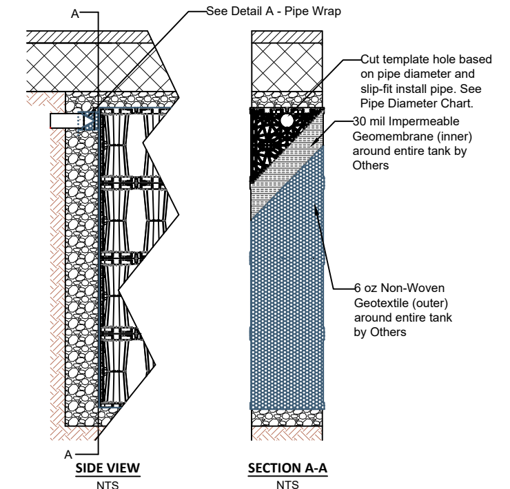
4 LAYER HD PIPE INSTALLATION NTS
