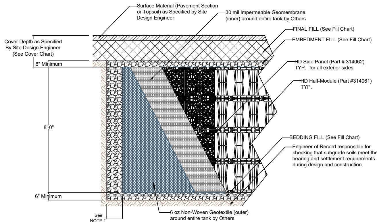
4 LAYER HD DETENTION CROSS SECTION NTS
