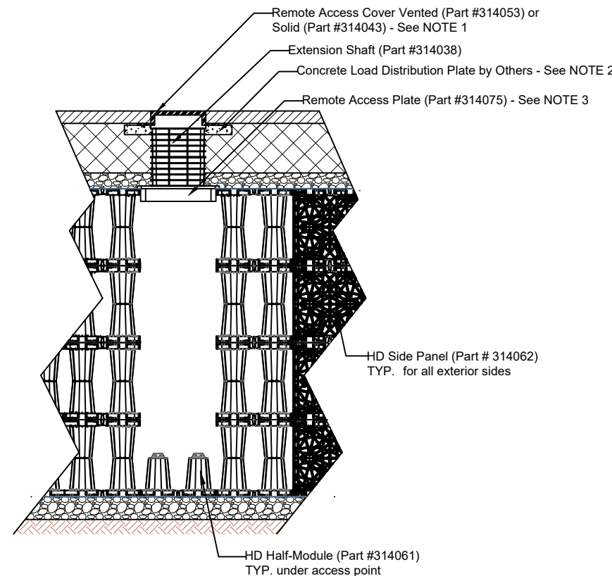
4 LAYER HD ACCESS POINT CROSS SECTION NTS
