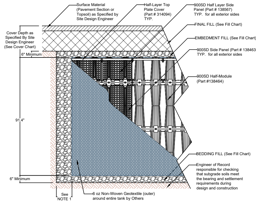
2.5 LAYER 900SD INFILTRATION CROSS SECTION NTS
