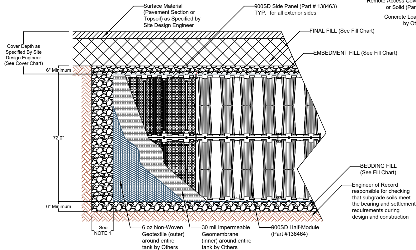
2 LAYER 900SD DETENTION CROSS SECTION NTS
