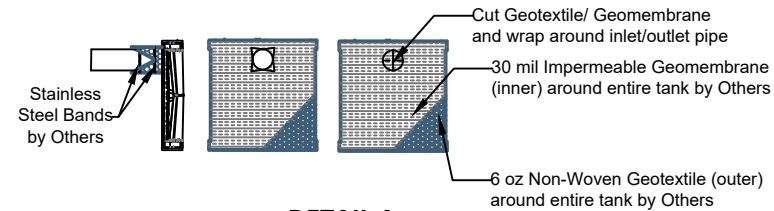
DETAIL A PIPE WRAP NTS
