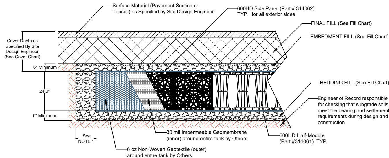
1 LAYER 600HD DETENTION CROSS SECTION NTS
