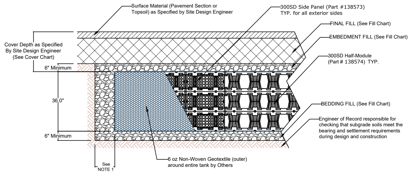
3 LAYER 300SD INFILTRATION CROSS SECTION NTS
