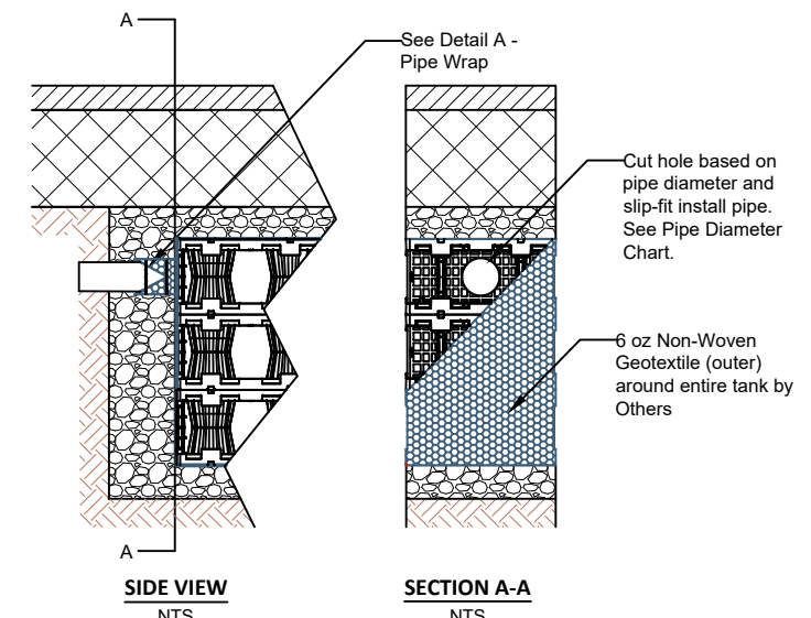
3 LAYER 300SD PIPE INSTALLATION NTS
