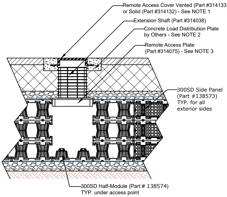
3 LAYER 300SD ACCESS POINT CROSS SECTION NTS
