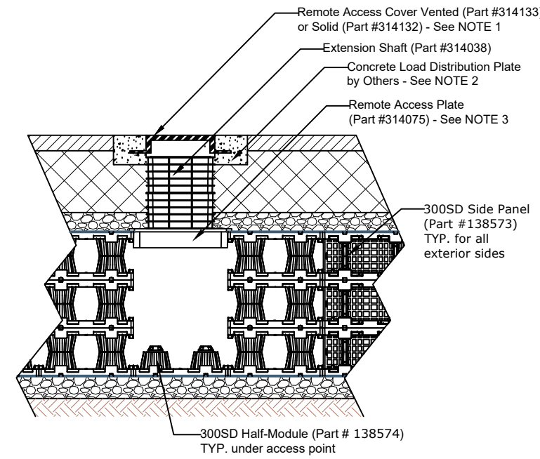
3 LAYER 300SD ACCESS POINT CROSS SECTION NTS
