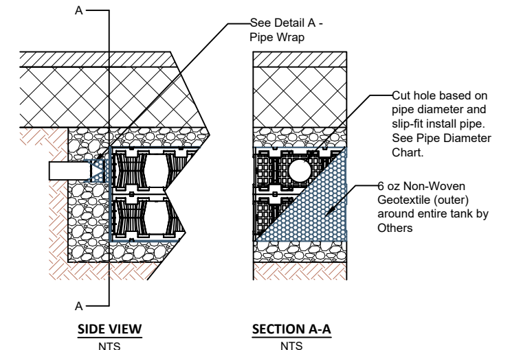
2 LAYER 300HD PIPE INSTALLATION NTS
