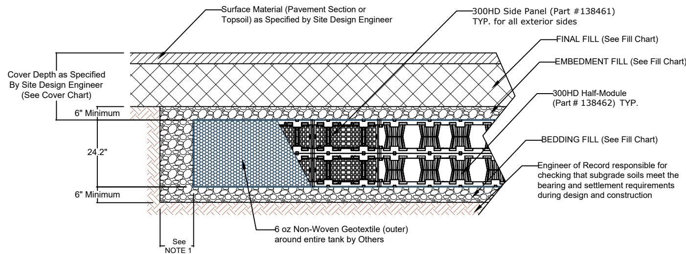
2 LAYER 300HD INFILTRATION CROSS SECTION NTS
