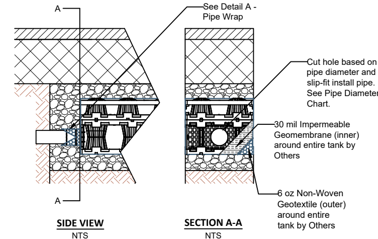
1.5 LAYER 300HD PIPE INSTALLATION NTS
