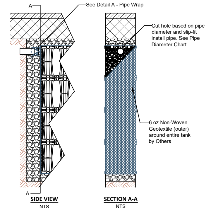
4 LAYER HD PIPE INSTALLATION NTS
