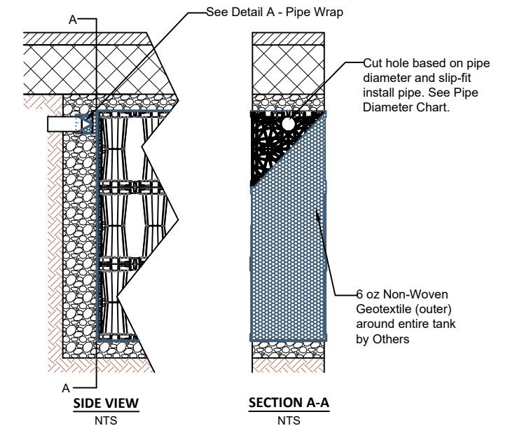
3 LAYER HD PIPE INSTALLATION NTS
