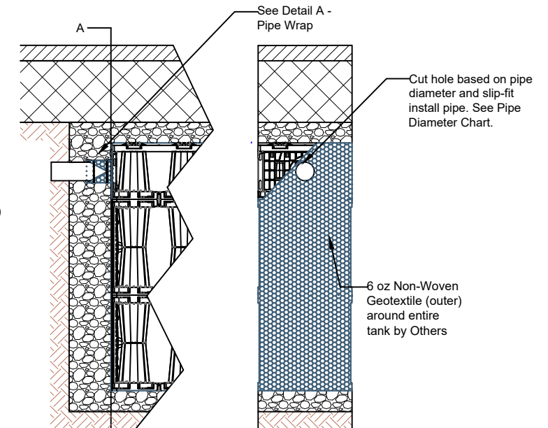
2.5 LAYER HD PIPE INSTALLATION NTS
