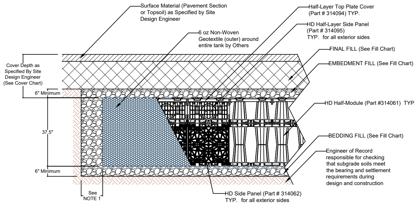
1.5 LAYER HD INFILTRATION CROSS SECTION NTS
