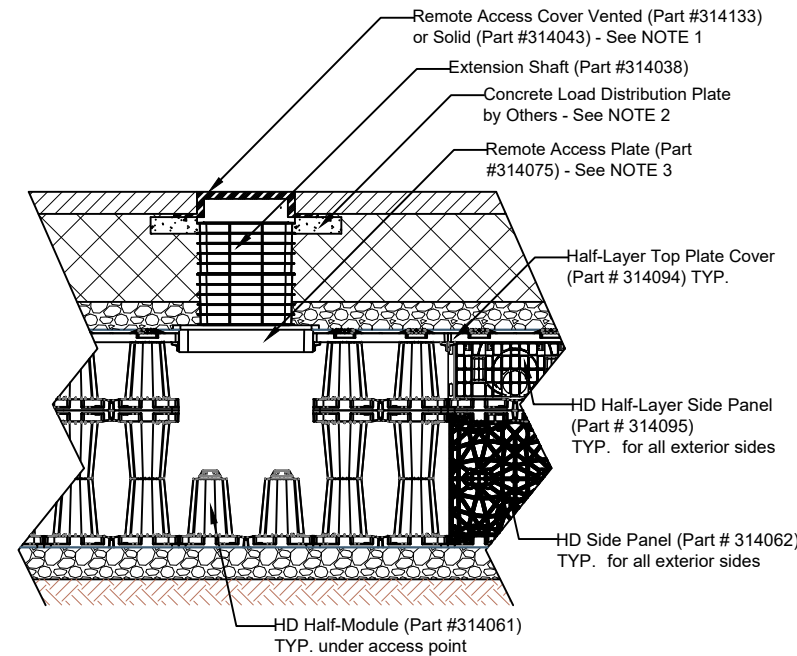
1.5 LAYER HD ACCESS POINT CROSS SECTION NTS
