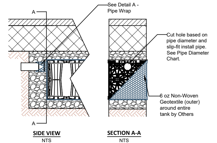
1 LAYER HD PIPE INSTALLATION NTS
