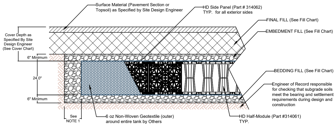
1 LAYER HD INFILTRATION CROSS SECTION NTS
