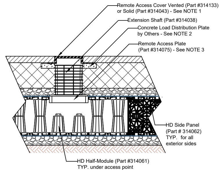
1 LAYER HD ACCESS POINT CROSS SECTION NTS
