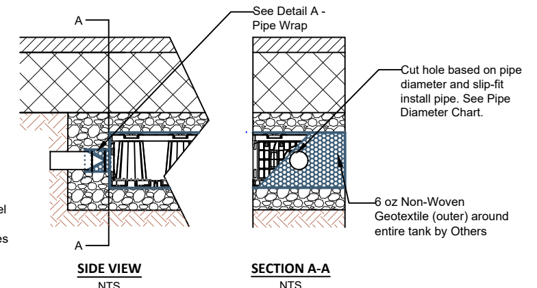
0.5 LAYER HD PIPE INSTALLATION NTS
