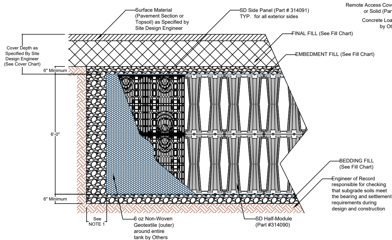
2 LAYER SD INFILTRATION CROSS SECTION NTS
