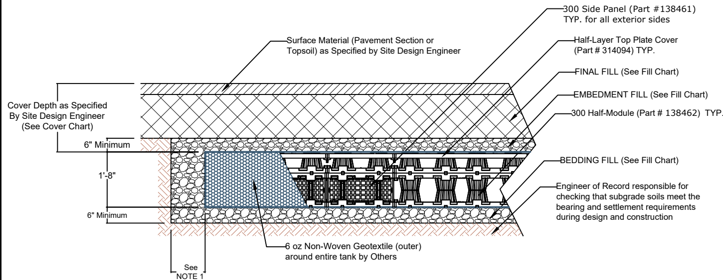
1.5 LAYER 300 INFILTRATION CROSS SECTION NTS
