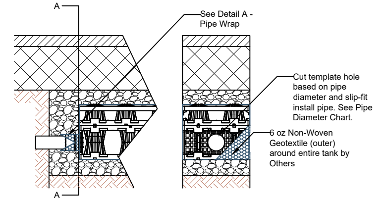
1.5 LAYER 300 PIPE INSTALLATION NTS
