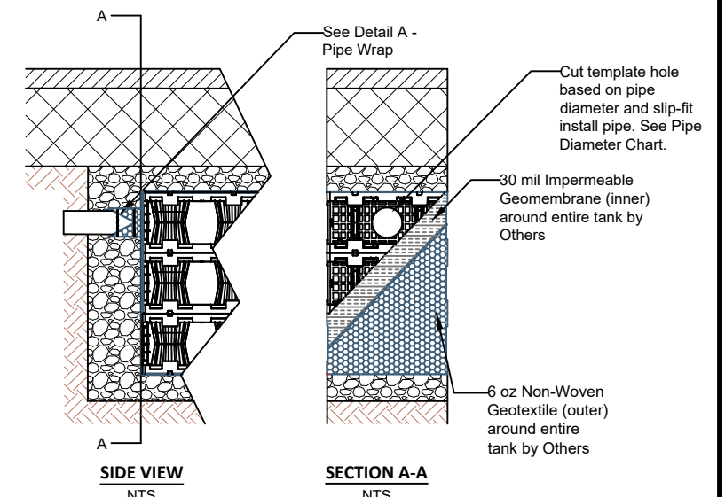
3 LAYER 300 PIPE INSTALLATION NTS
