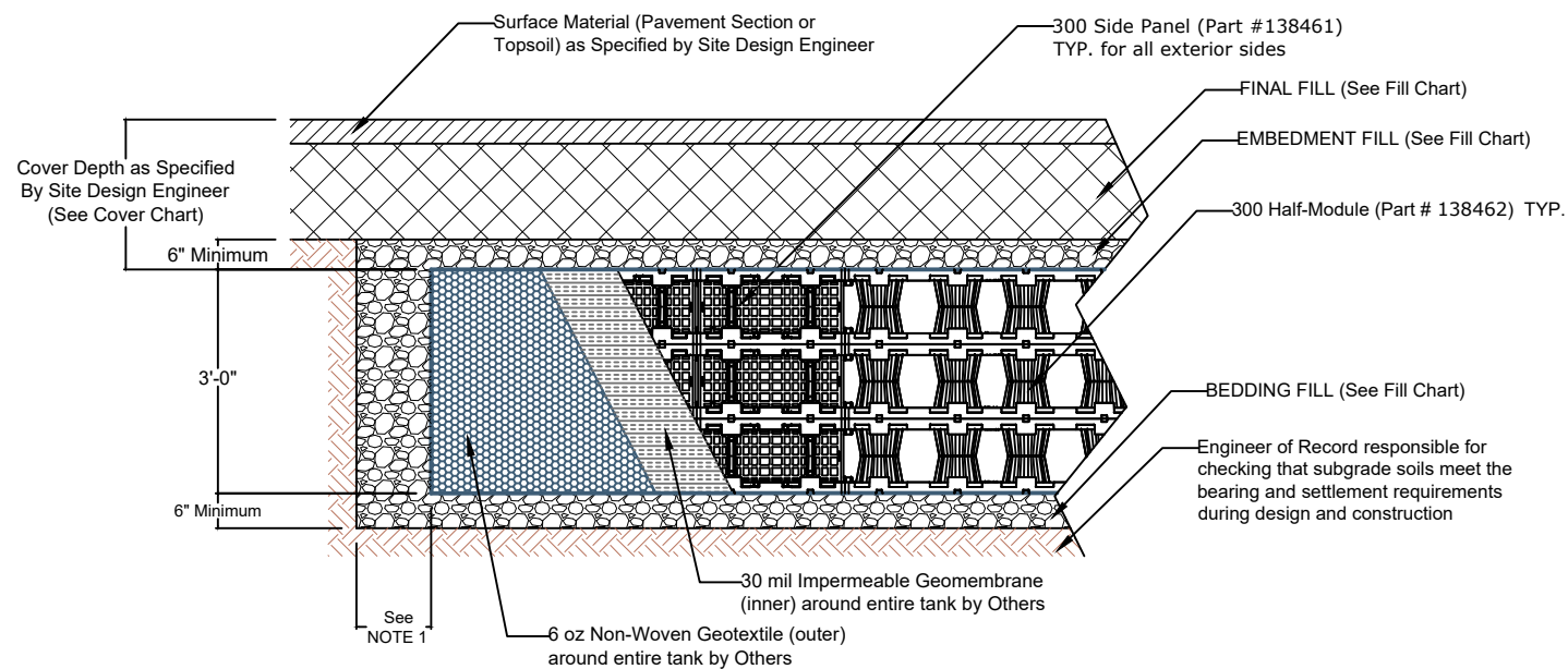
3 LAYER 300 DETENTION CROSS SECTION NTS
