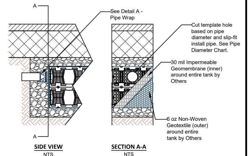
2 LAYER 300 PIPE INSTALLATION NTS
