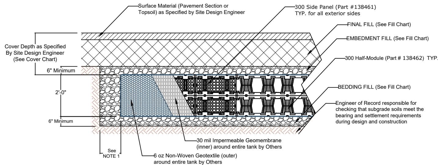
2 LAYER 300 DETENTION CROSS SECTION NTS
